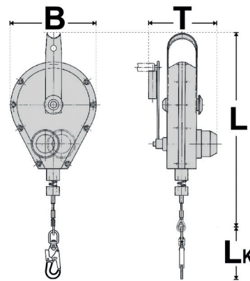
IKV 33 (ANSI Z.359.1-2007; CSA Z259.12-2011) with fall indicator
